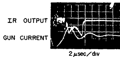
Fig. 57. Interferometer measured gun plasma density at high transverse field B = 7.5 kG
