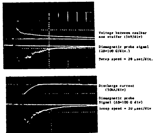
Fig. 43. Diamagnetic field signal obtained with probe positioned in plane 25 cm from midplane and 16 cm from axis of machine.
