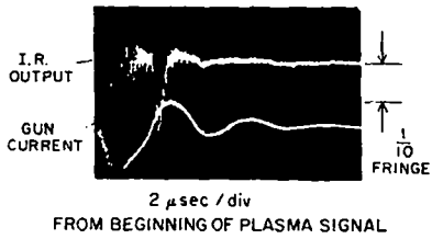
Fig. 56. Interferometer measured density of gun plasma in transverse field B = 5 kG.
