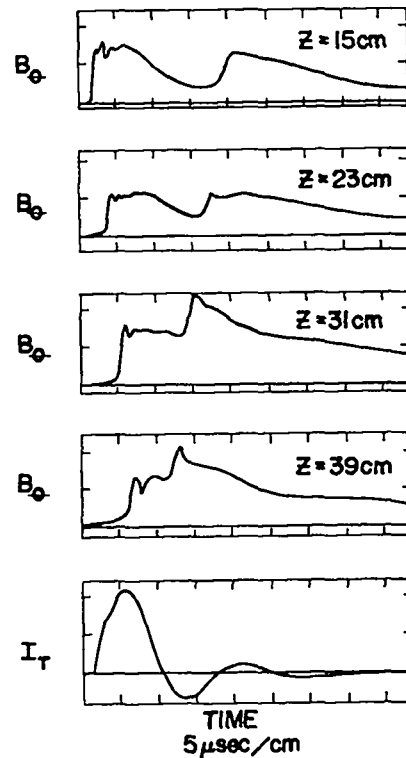
Fig. 31. Magnetic probe traces at four axial positions; the lower trace is the total discharge current.
